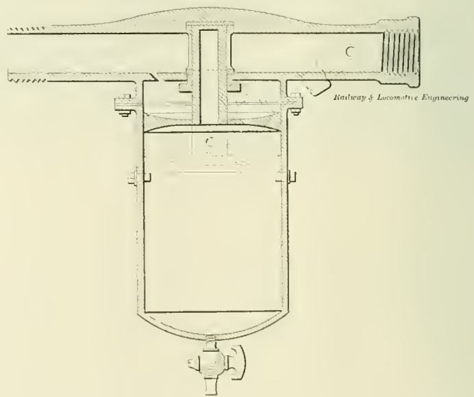
SECTIONAL VIEW OF MORRISON AUTOMATIC VALVE.
